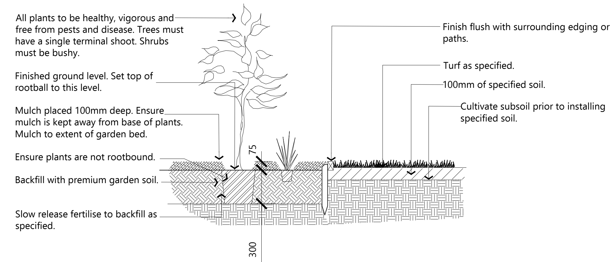
Mass planting and turf Detail Scale 1:20
