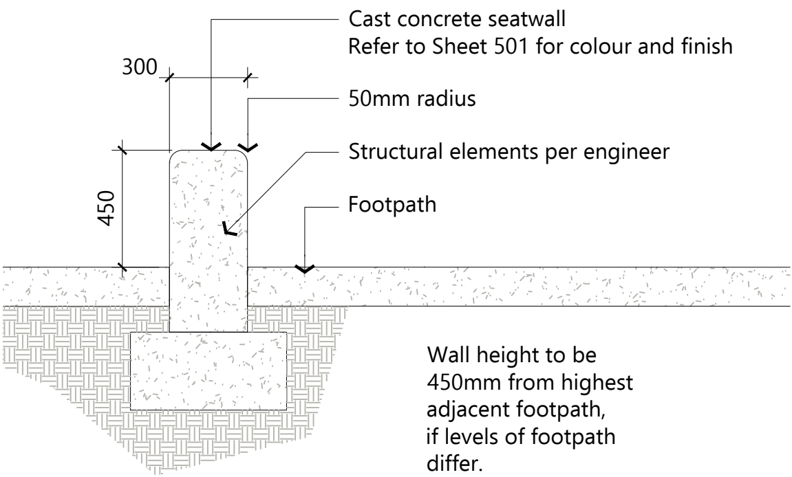
Concrete Seat Wall Detail Scale 1:20
