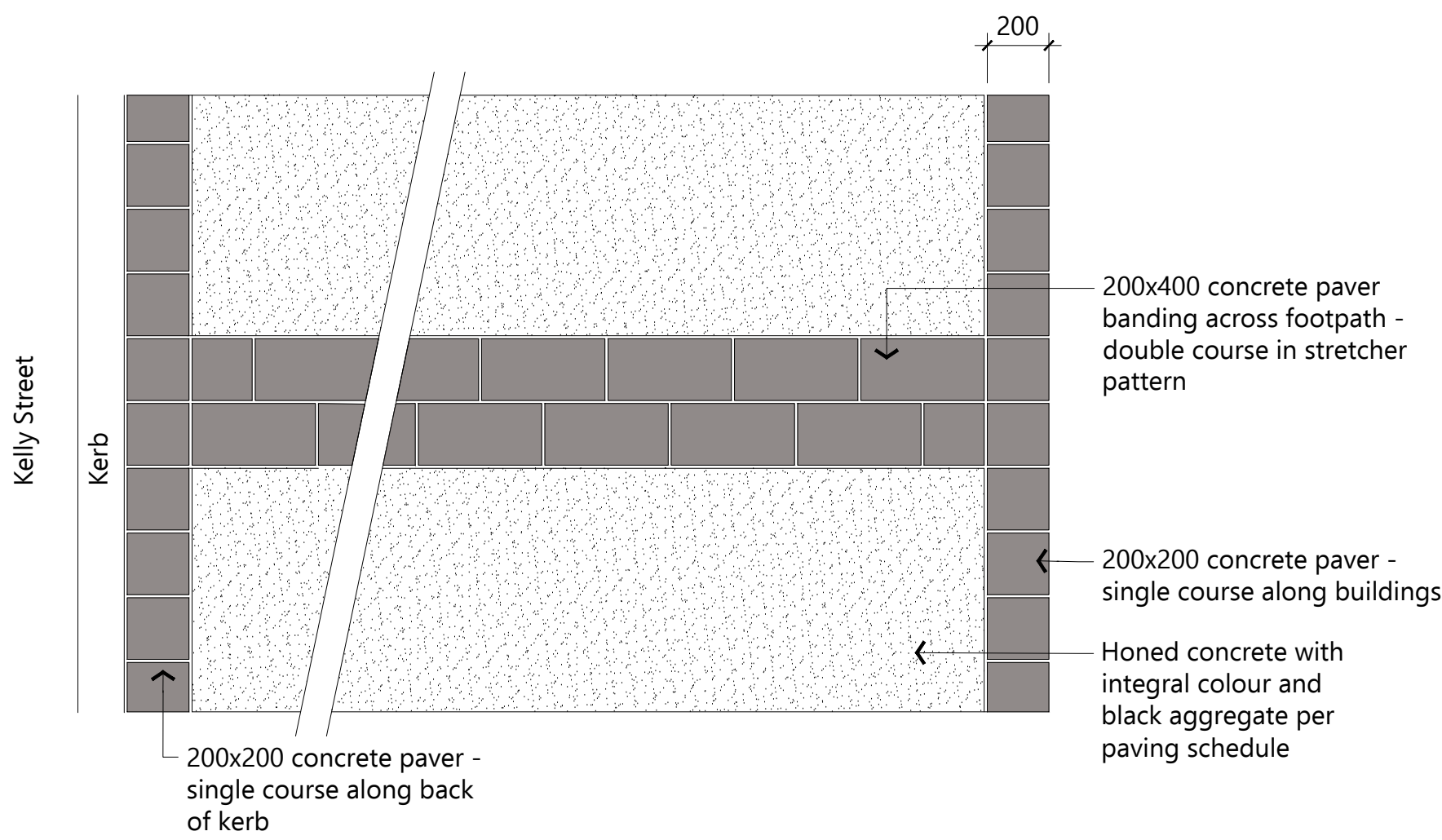
Footpath paving layout Plan Scale 1:20
