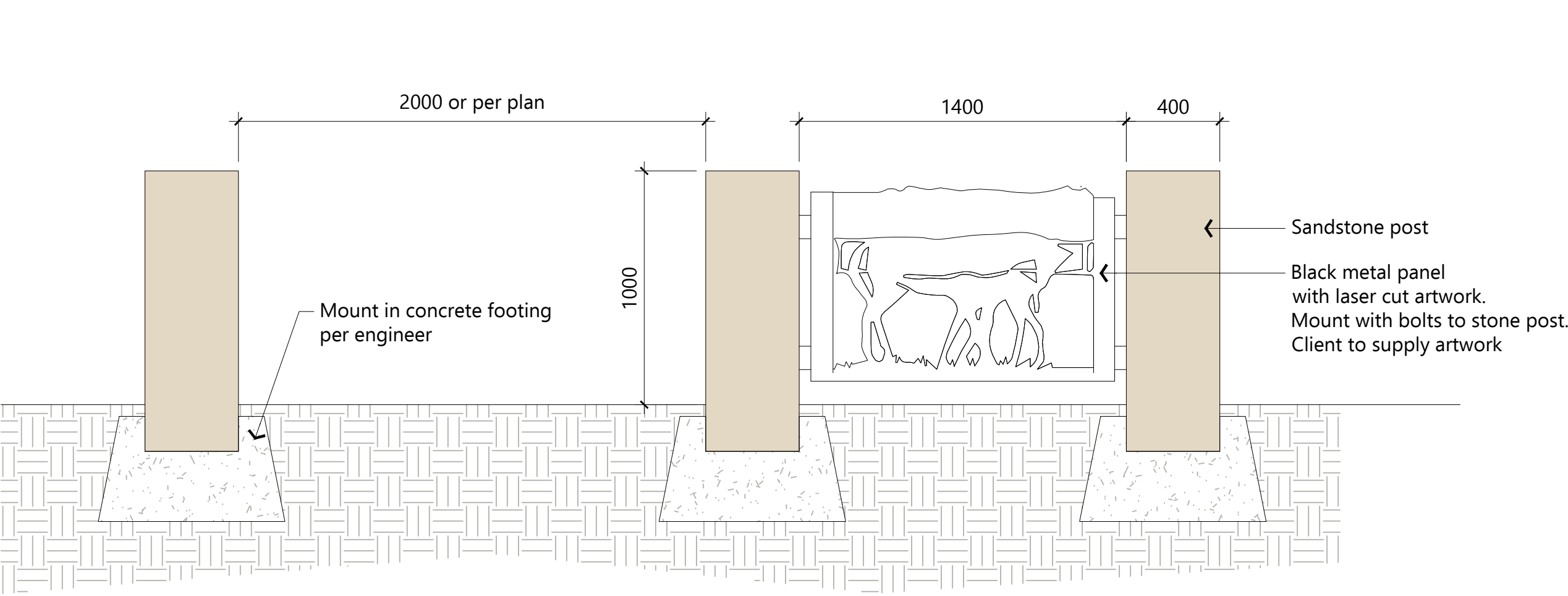
Thematic Fence - Stone Elevation Scale 1:20
