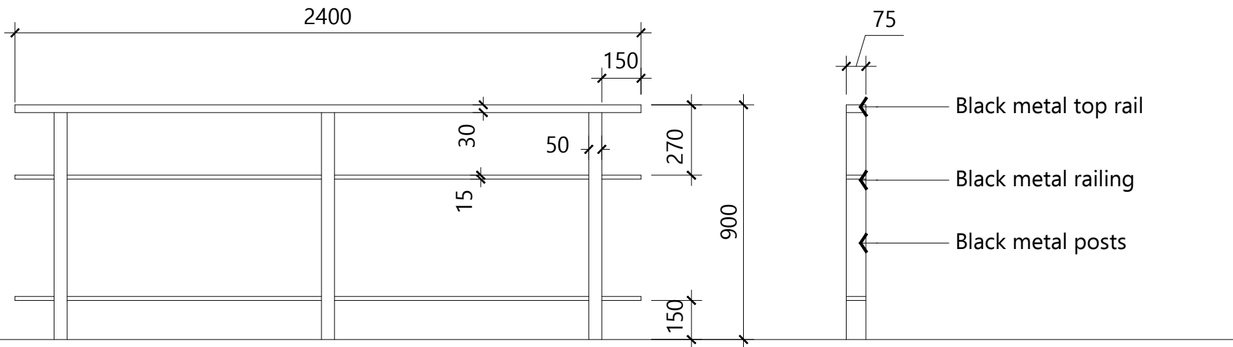
Black Metal Containment Fence Elevation Scale 1:20
