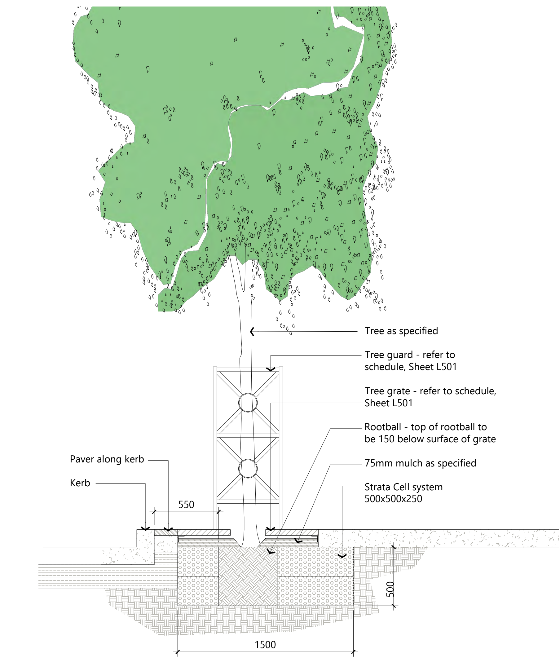
Tree planting with tree grate Detail Scale 1:20
